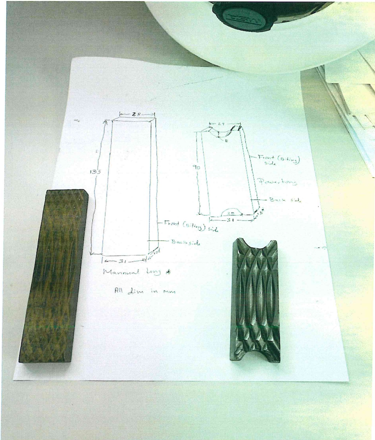
Picture 2: The front (biting) side of the tong dies
